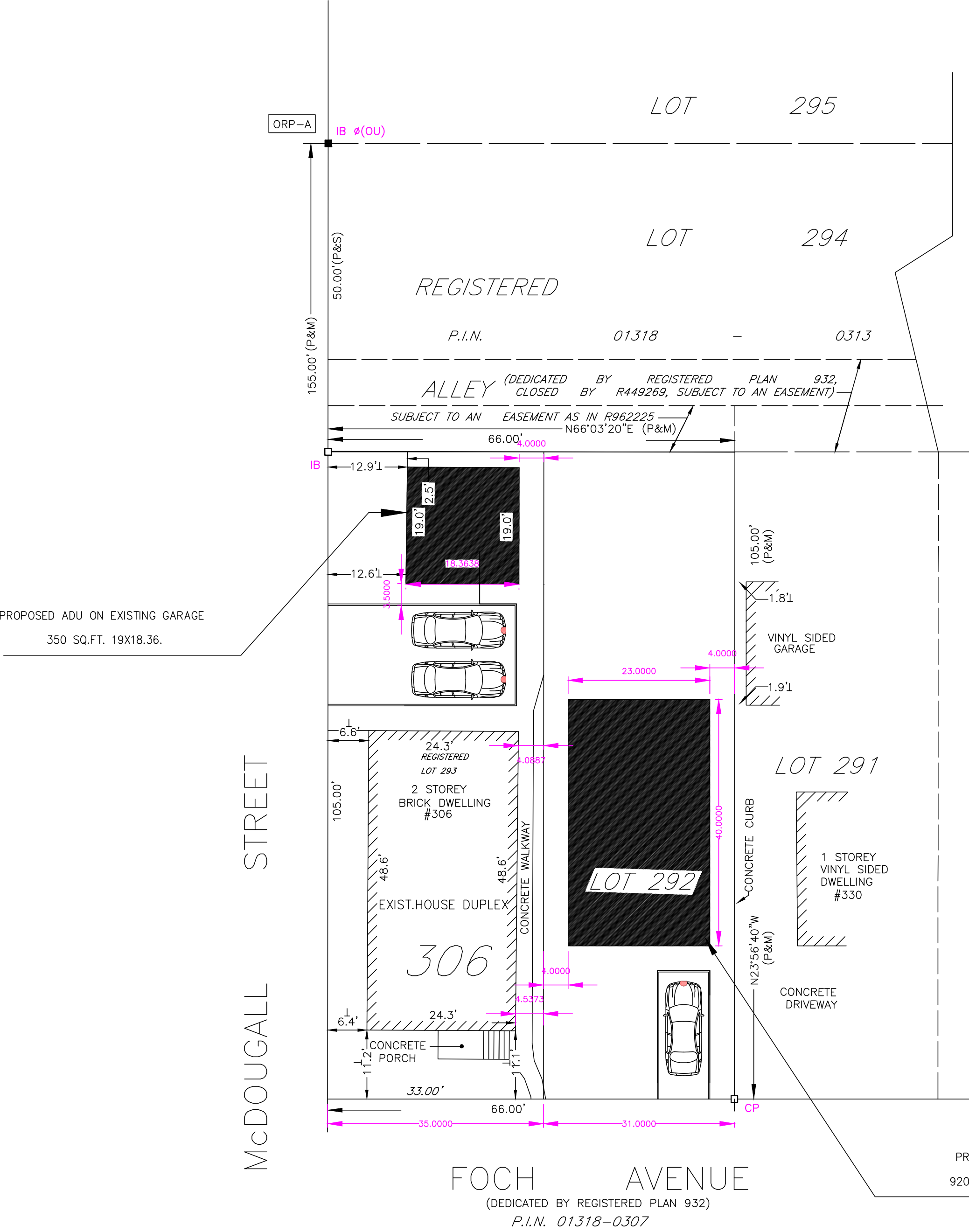
PROPOSED NEW BUILD SINGLE DETACHED
