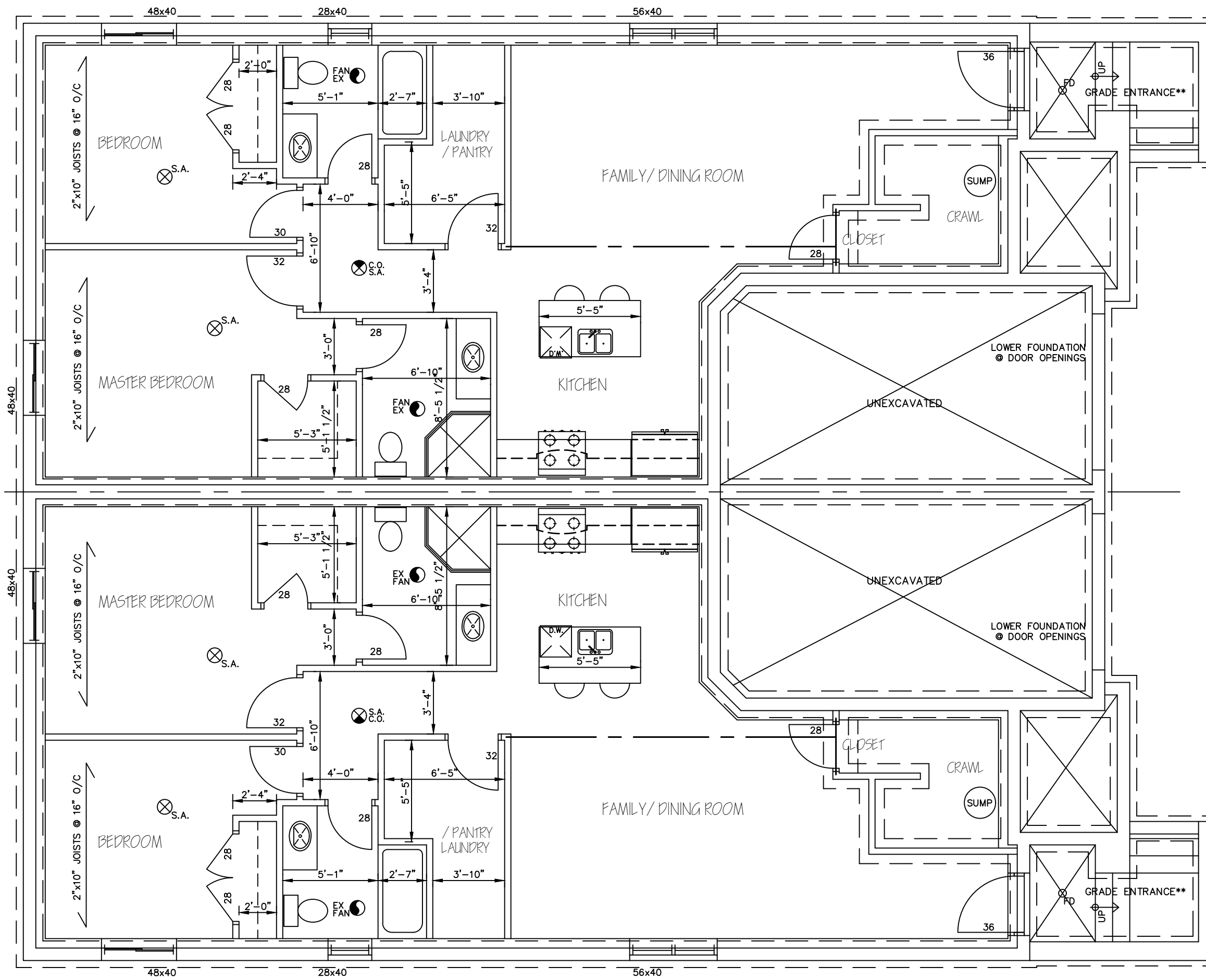
FLOOR AREA 1158 SF - EACH SIDE
