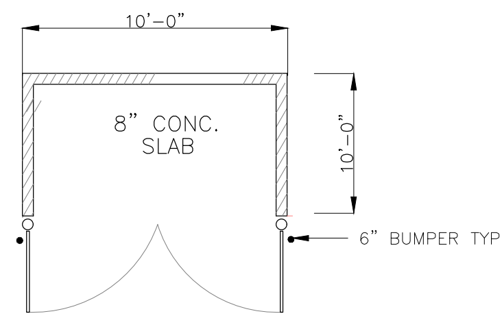
DUMPSTER PLAN
