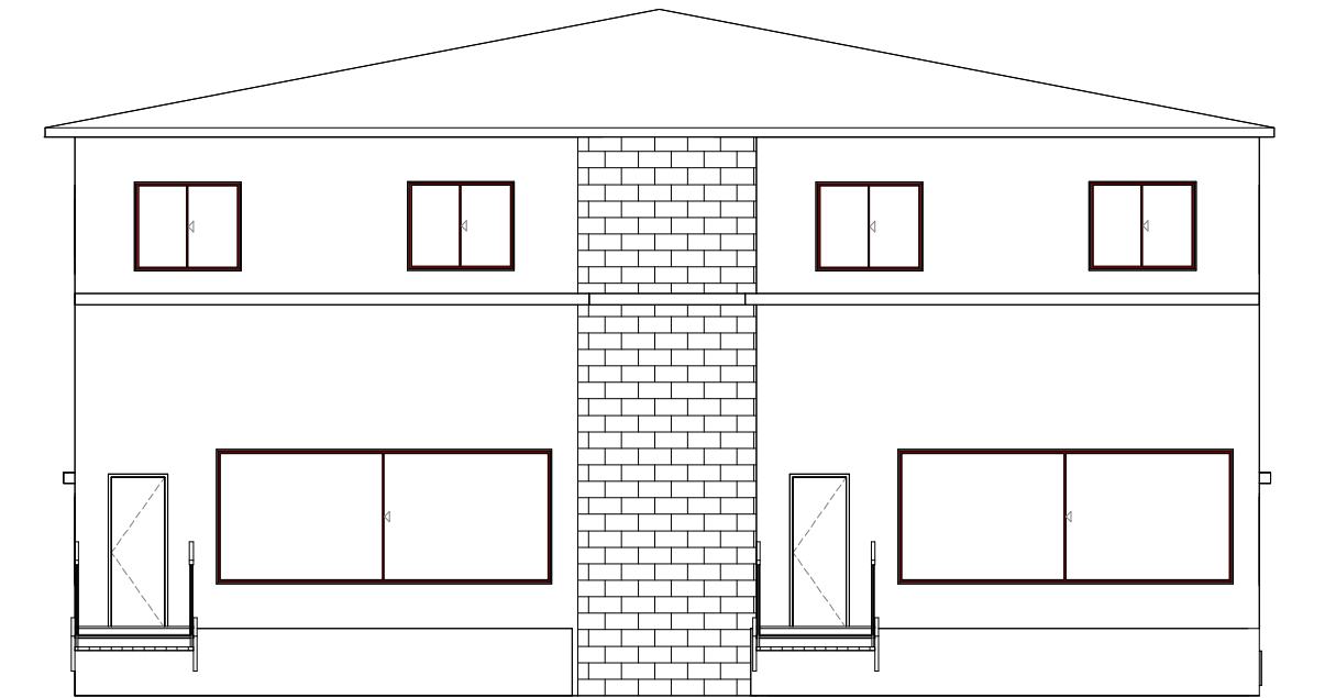
REAR ELEVATION
