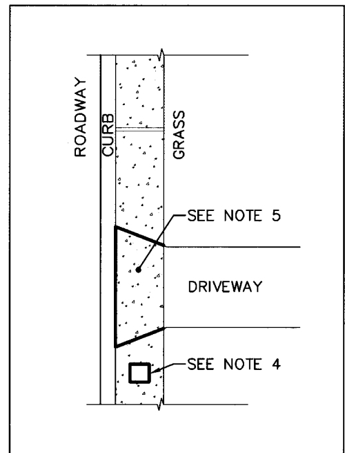
SCENARIO 2 LESS THAN 0.6m SEPARATION BETWEEN SIDEWALK AND BACK OF CURB
