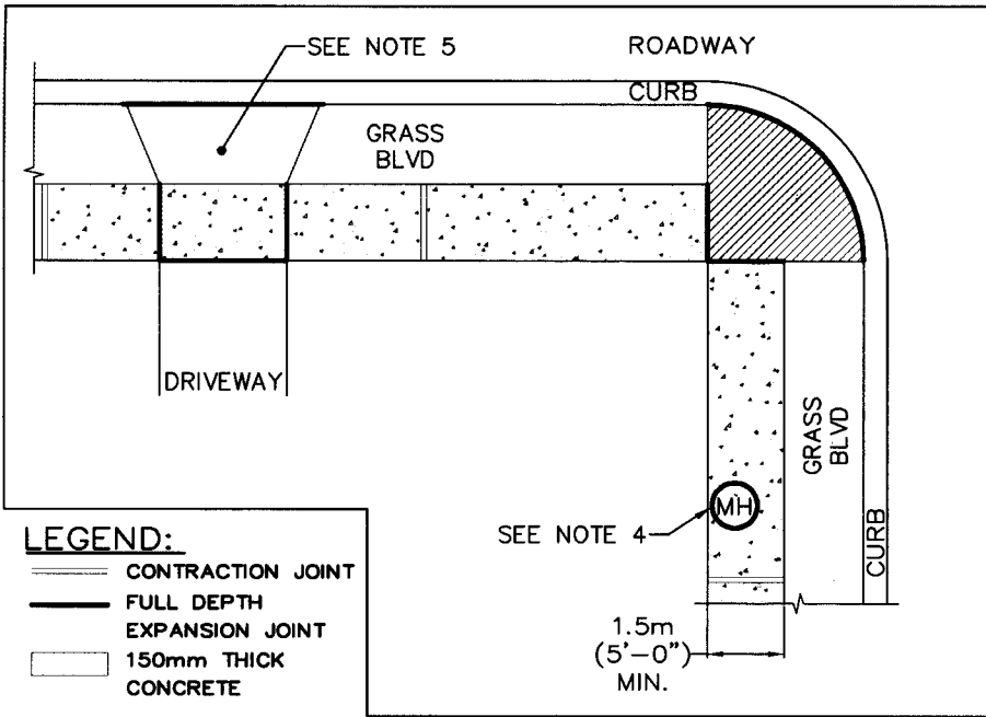
SCENARIO 1 MORE THAN 0.6m SEPARATION BETWEEN SIDEWALK AND BACK OF CURB
