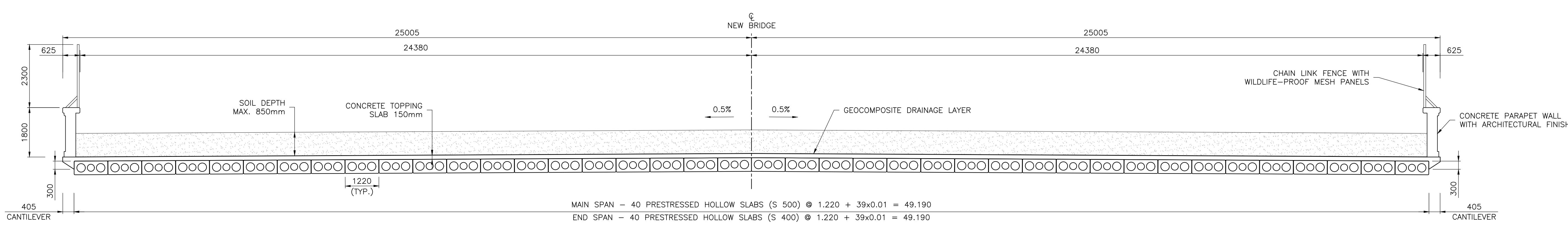
SPAN SECTION SCALE 1:75
