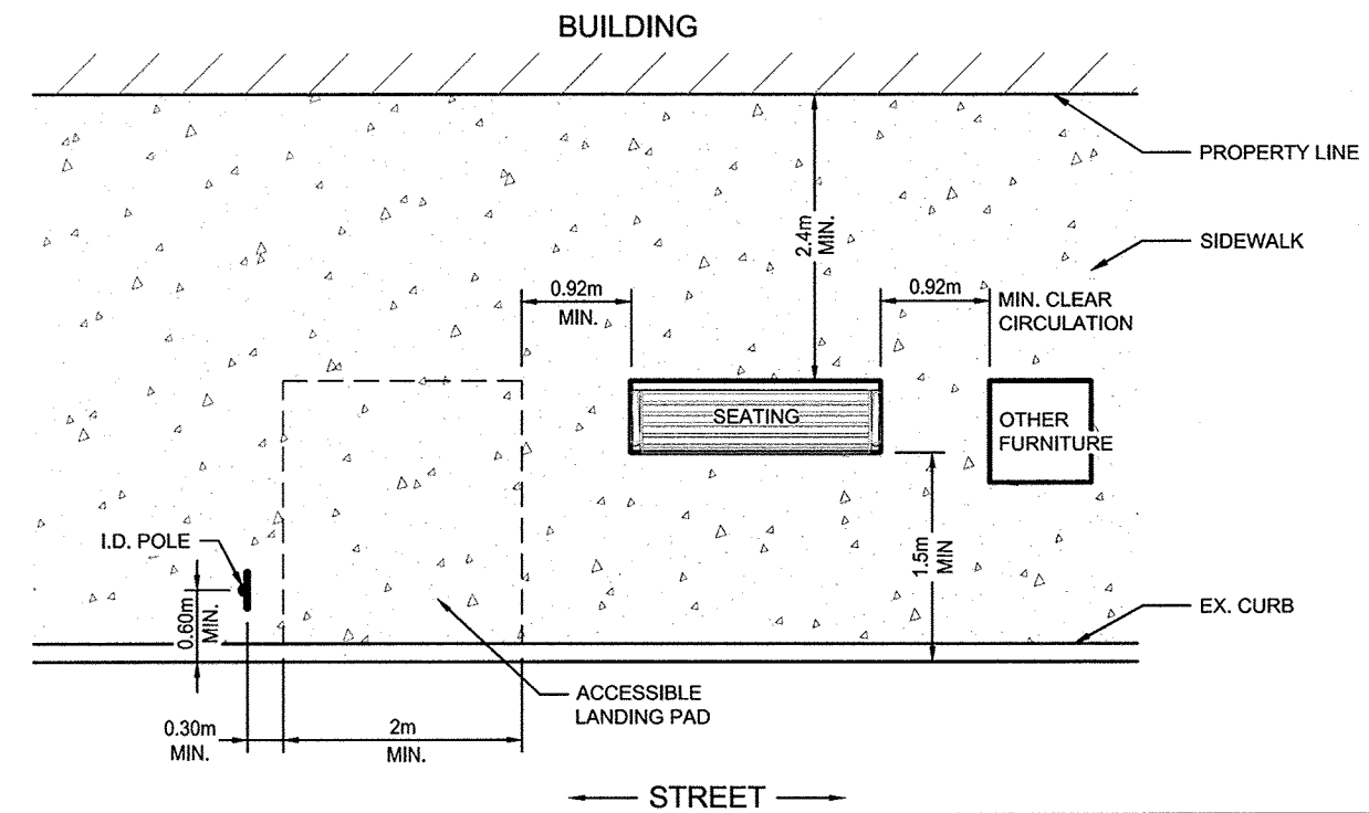
CASE 2: SIDEWALK ADJACENT TO CURB
