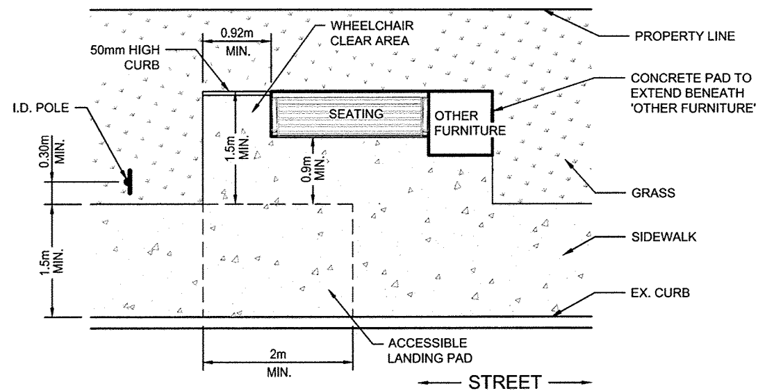
CASE 1: SIDEWALK ADJACENT TO CURB
