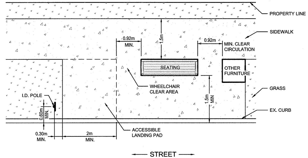
CASE 2: SIDEWALK WITH BLVD
