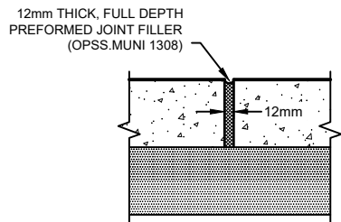
ISOLATION/EXPANSION JOINT
