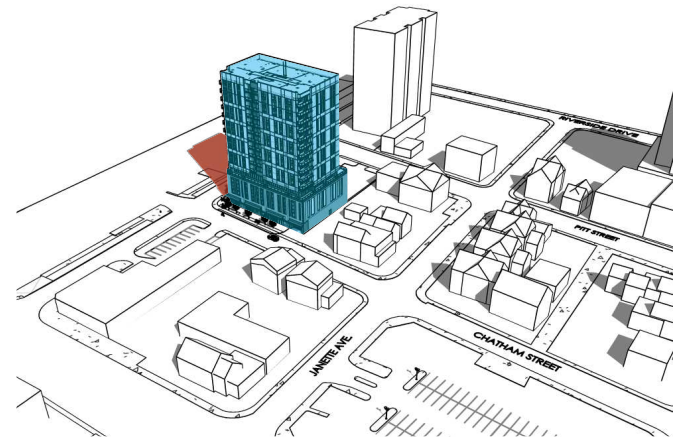
9:00 AM SUMMER SOLSTICE
