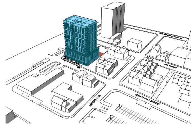
12:00 PM SUMMER SOLSTICE
