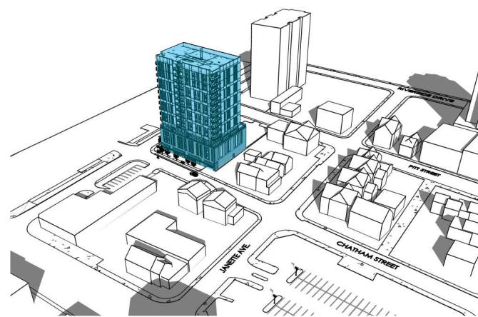
9:00 AM FALL EQUINOX
