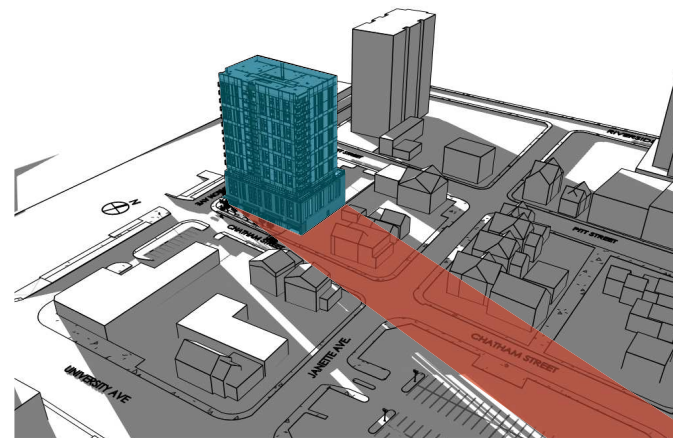
7:45 PM (SUNSET) SPRING EQUINOX
