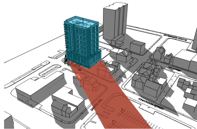
6:00 PM SUMMER SOLSTICE
