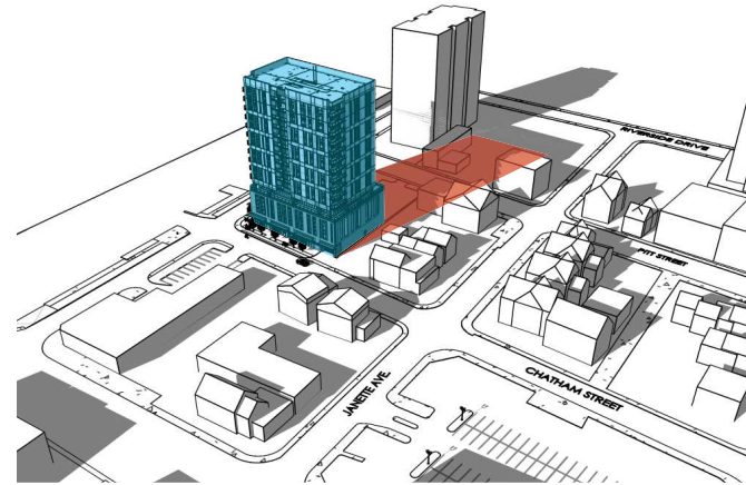
12:00 PM WINTER SOLSTICE
