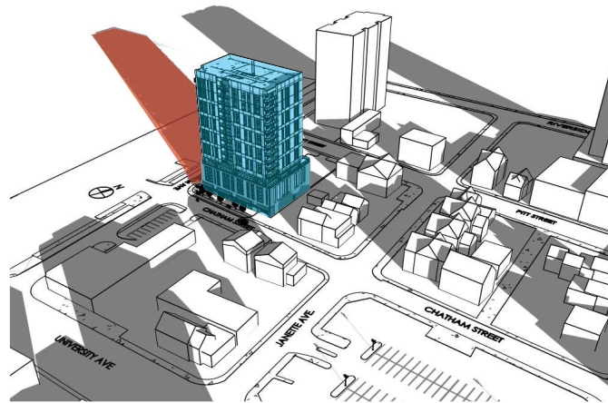
7:20 AM (SUNRISE) FALL EQUINOX
