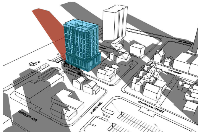
7:30 AM (SUNRISE) SPRING EQUINOX
