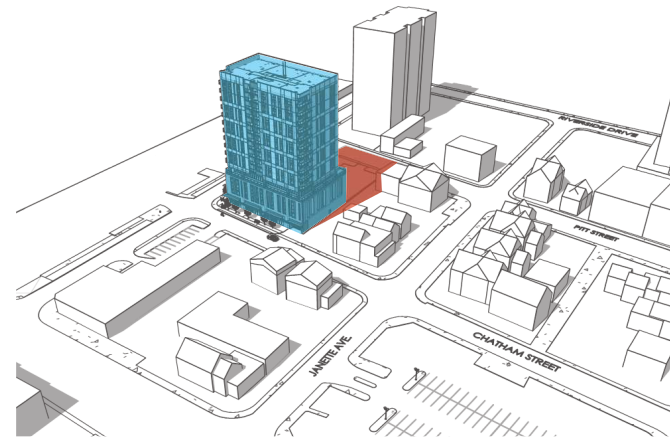
12:00 PM SPRING EQUINOX
