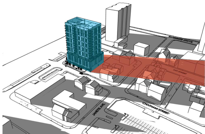
4:00 PM WINTER SOLSTICE
