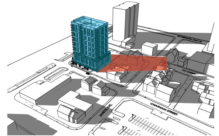
3:00 PM WINTER SOLSTICE
