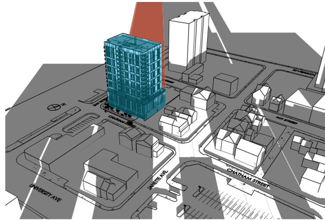
8:00 AM (SUNRISE) WINTER SOLSTICE
