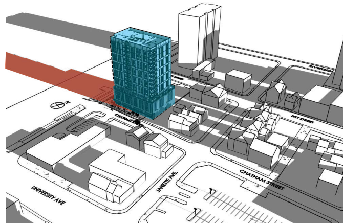
6:00 AM (SUNRISE) SUMMER SOLSTICE
