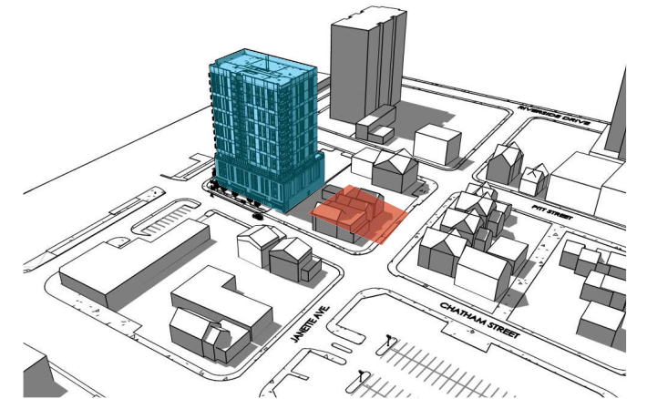
3:00 PM SUMMER SOLSTICE
