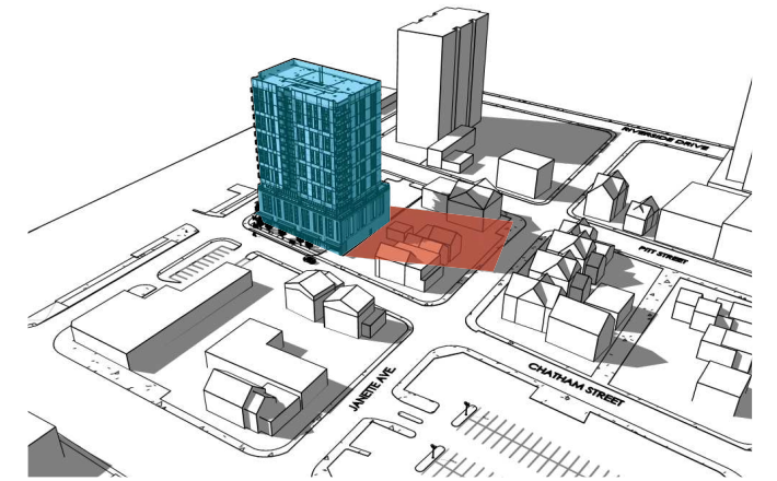
3:00 PM SPRING EQUINOX
