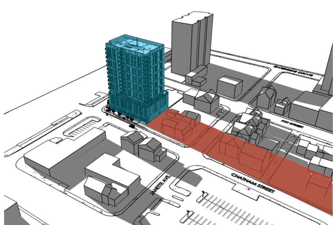
5:00 PM FALL EQUINOX
