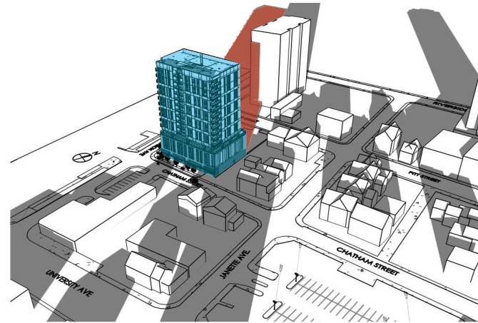
9:00 AM WINTER SOLSTICE
