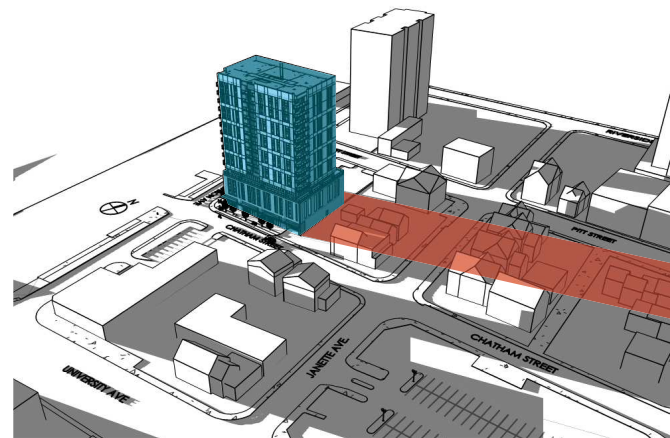
5:00 PM (SUNSET) WINTER SOLSTICE
