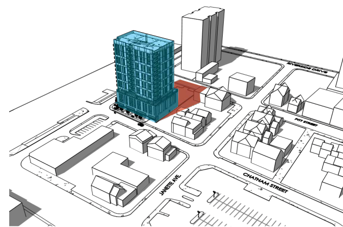
12:00 PM FALL EQUINOX
