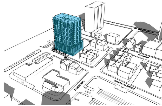
9:00 AM SPRING EQUINOX
