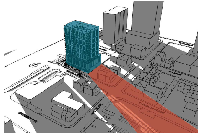
7:30 PM (SUNSET) FALL EQUINOX
