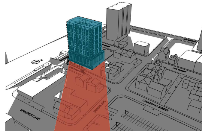
9:00 PM (SUNSET) SUMMER SOLSTICE
