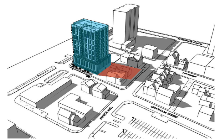
3:00 PM FALL EQUINOX
