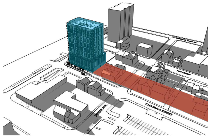
5:00 PM SPRING EQUINOX
